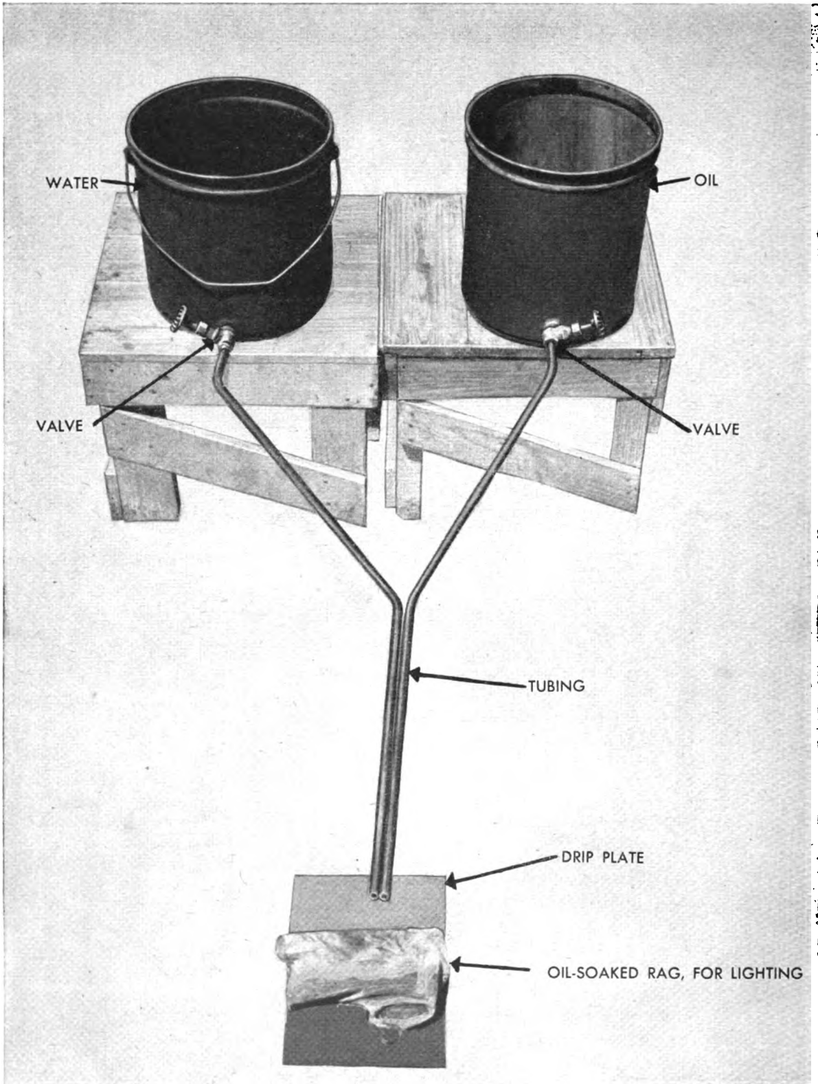
Figure 60. Detail of oil-and-water burner.
