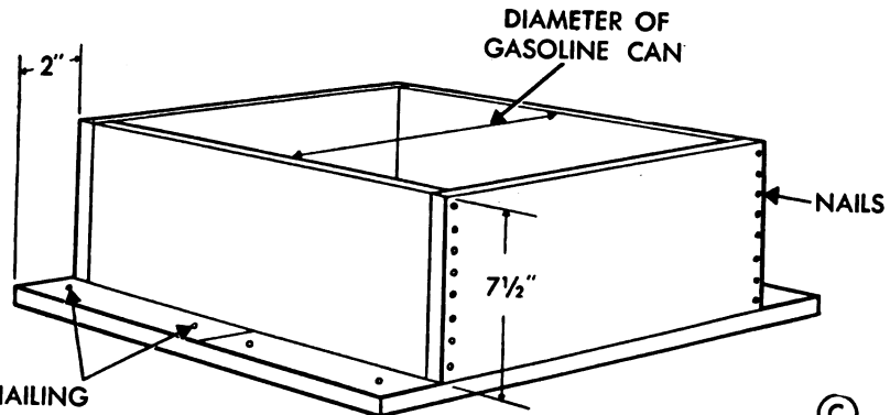
Figure 42. Detail of field range and fuel can installation in railway kitchen car.
