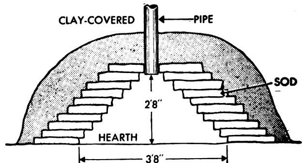
Figure 83. Sod oven.
