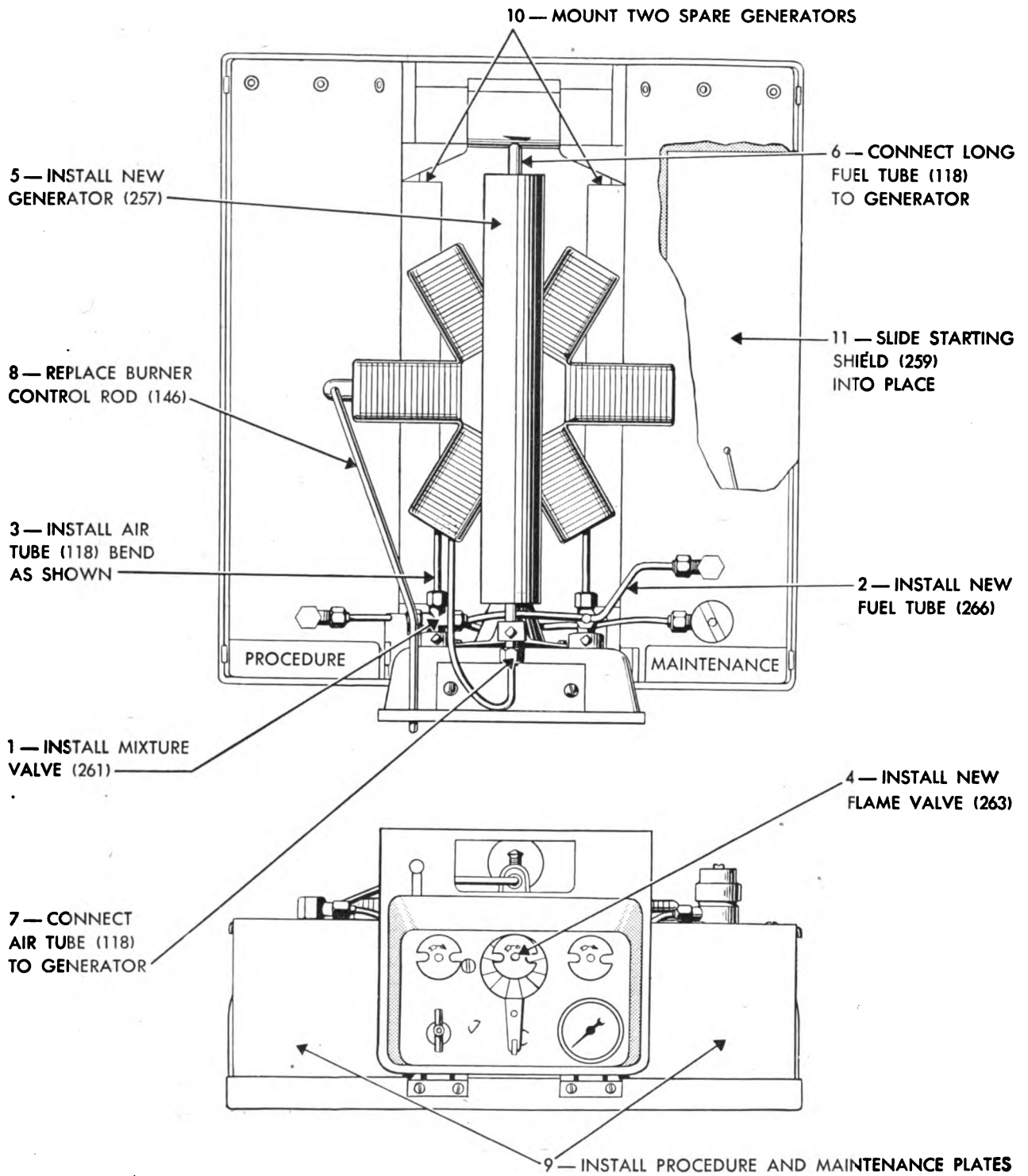
Figure 51. Installation of set, conversion, No. 2 (simplified) (65-J-2377).
