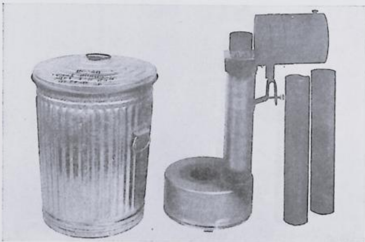
Figure 1. Heater, immersion type, for can, corrugated, QM stock No. 65-J-1911-50.
