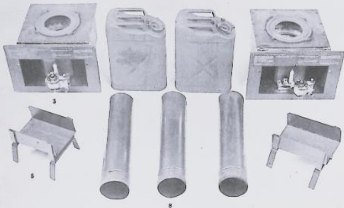
FIGURE 1.—Outfit burner, pot type, used, lake, field, M-1812, complete.
