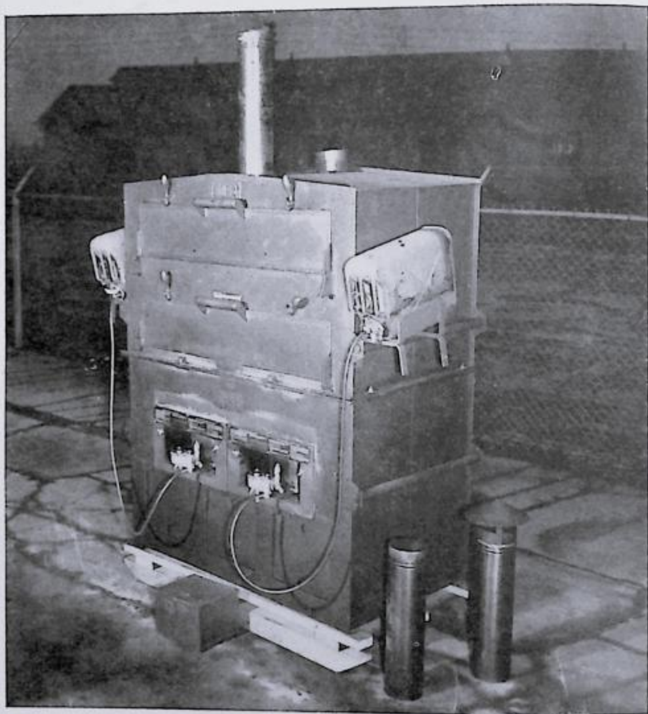
FIGURE 2.—Outfit, Burner, Pot Type, Oven, Bake, Field (M-1942) Assembled in Oven, Bake, Field (M-1942).
