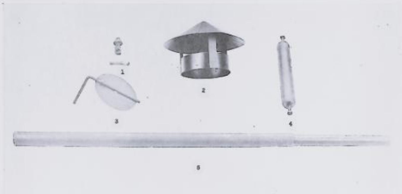
FIGURE 1.—Spare Parts For Owen, Babo, Field, M-1942.
