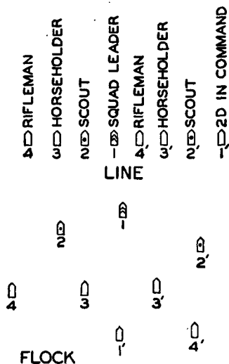
Figure 9. Squad formations.
