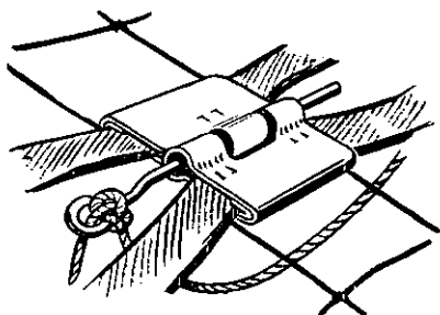
FIGURE 67 (1). — Quick-release device—hinge and pin.
