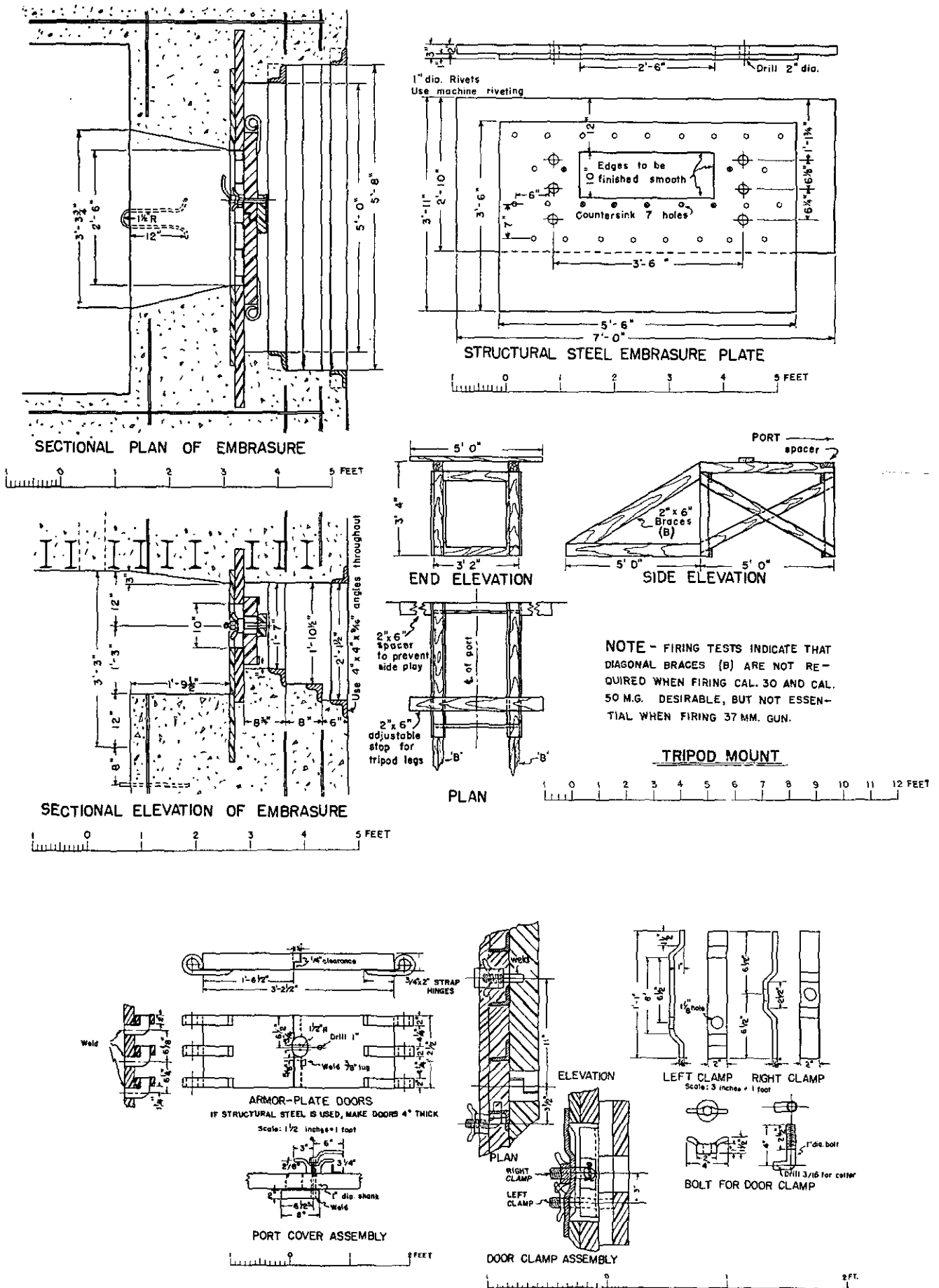
FIGURE 99.—Section and details of embrasure and tripod mount, light shellproof machine-gun emplacement.
