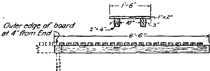
FIGURE 43.—Trench board.
