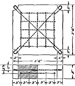
Concrete Beam
