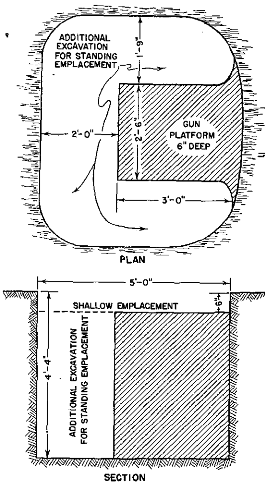
FIGURE 91.—Light machine-gun emplacement.
