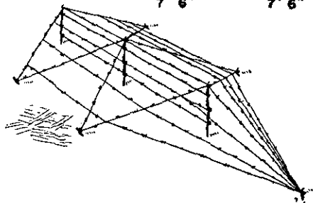
FIGURE 76.—Double-apron fence, 6- and 3-pace.
