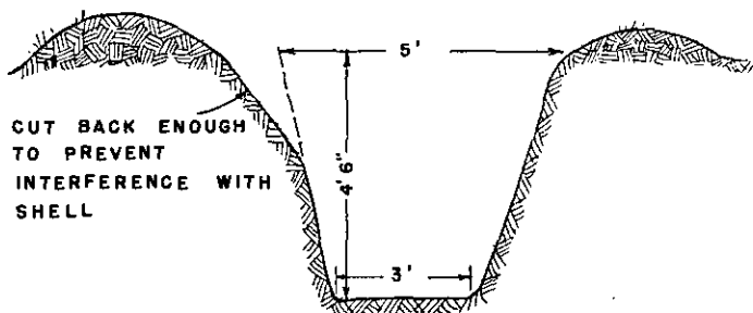
FIGURE 94.—Emplacement for 81-mm mortar (ammunition niches to be dug into side of pit).
