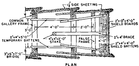
Figure 107. Use of shield in driving sheeting in loose, caving soil.
