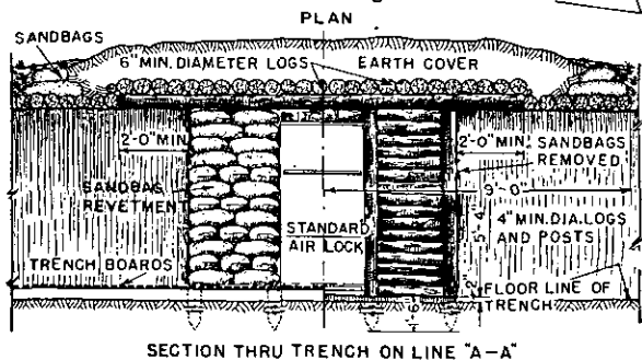
Figure 86. Cut-and-cover shelter constructed of logs.
