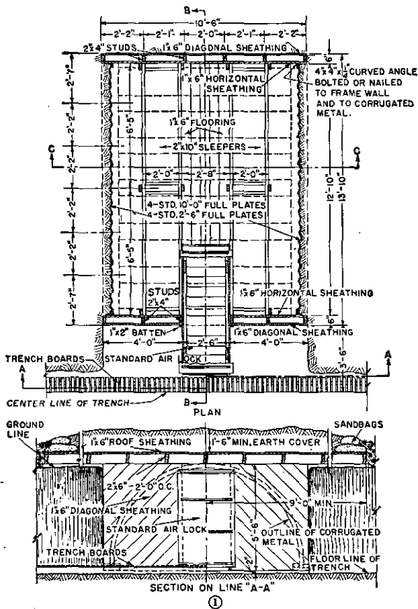
Figure 88. Cut-and-cover shelter constructed of semicircular corrugated metal arches.
