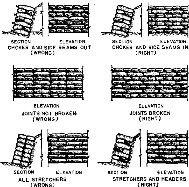
Figure 11. Sandbag revetment.
