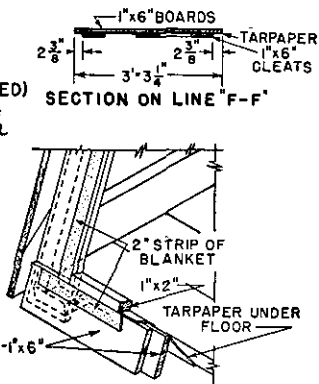
ISOMETRIC DETAIL OF J (GAS CURTAIN REMOVED)
