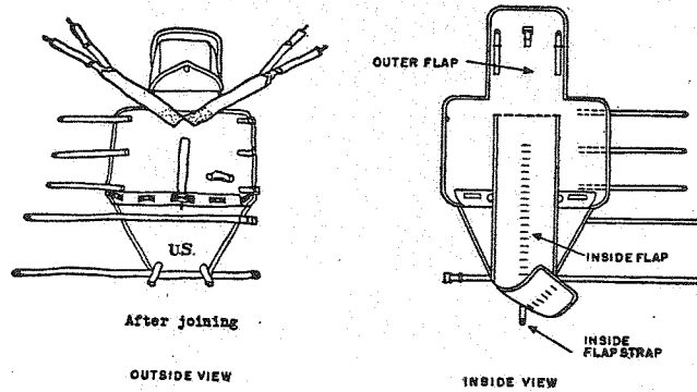
Figure 9. Haversack and pack carrier.
