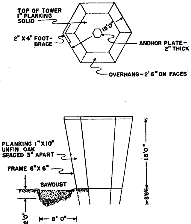
Figure 27. Belay tower.
