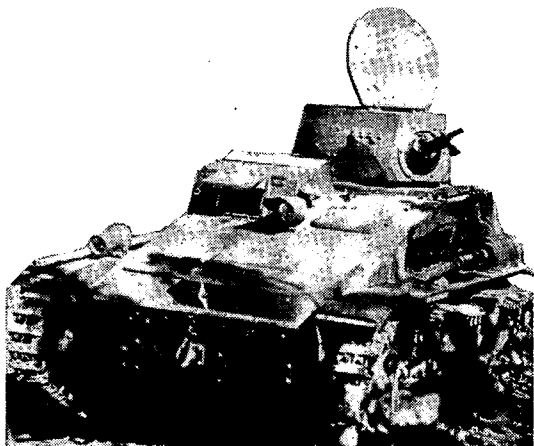
TANKETTE, ISHIKAWAJIMA, M 2592 (1932)
