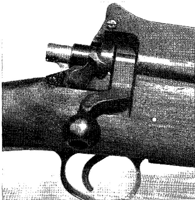
FIGURE 10.—Positions of safety lock—Continued.
