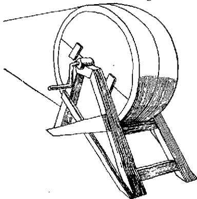
FIGURE 60.—Cable drum.
