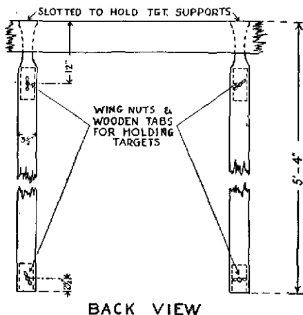
SUPPORTS FOR INDIVIDUAL FIRING TARGETS FIGURE 59.—Nonoverhead target carrier.
