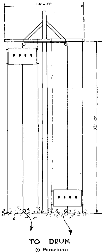
FIGURE 57.—Types of miniature range targets—Continued.
