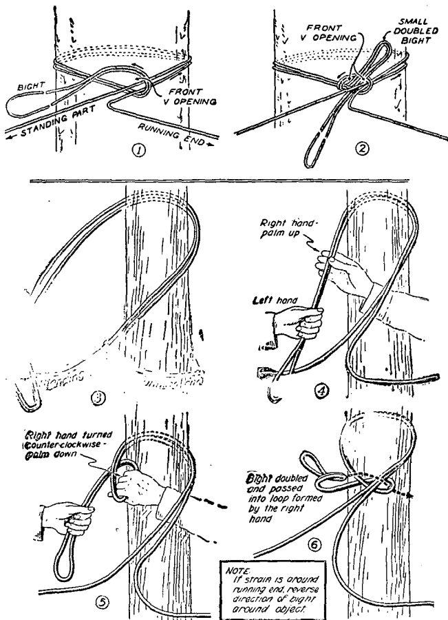
Figure 33. Loop knot ties, showing only one of the two conductors.
