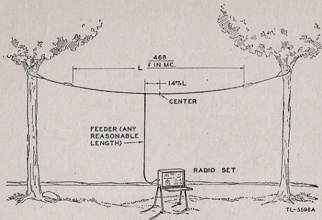
Figure 4. Single-wire-fed Hertz antenna.
